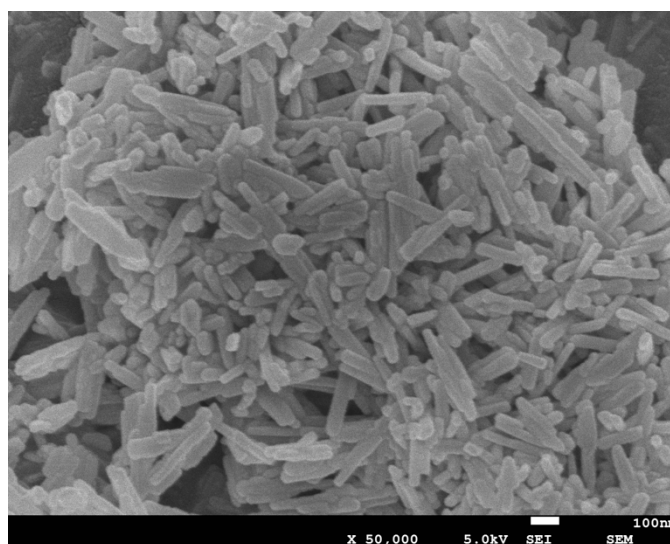
Typical SEM Image of ACS Material ZSM-23, Type A
