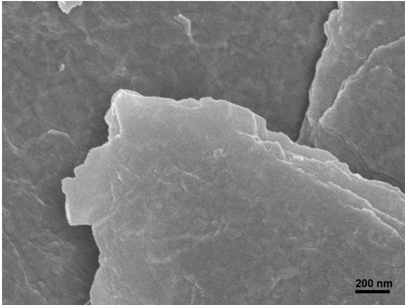
Typical SEM Image of ACS Material Pyrolytic Graphite Powder
